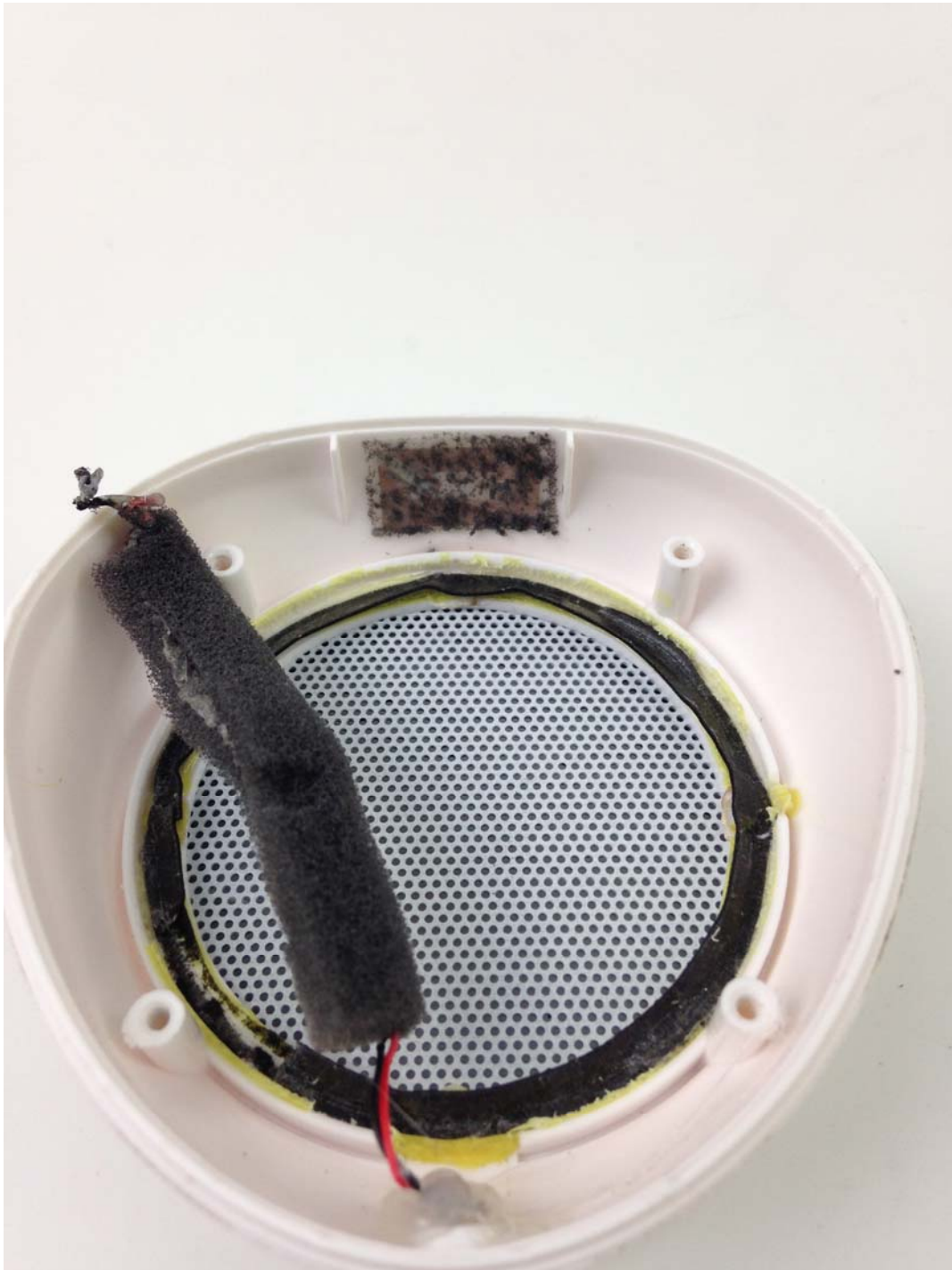
INTERNAL PHOTO OF SAMPLE – 8
