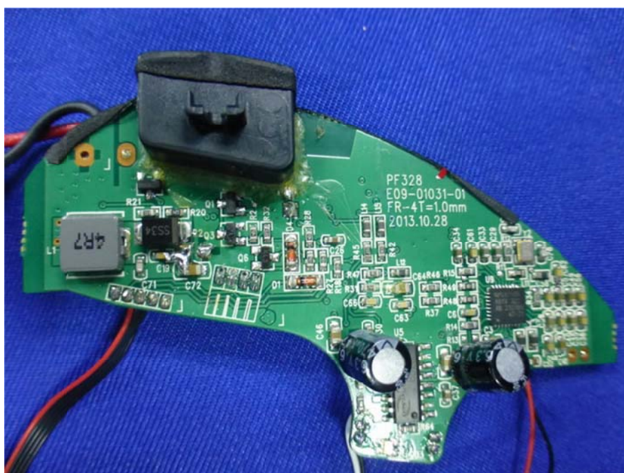
Figure 6 EUT Internal Photo
