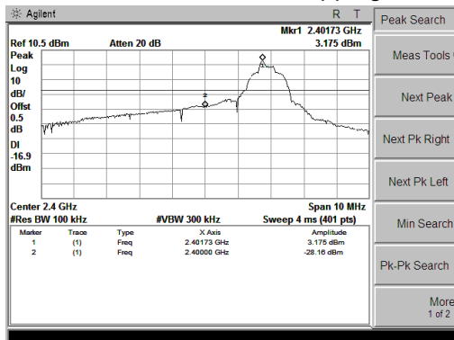
π/4-DQPSK Mode, Non-Hopping
