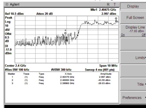
π/4-DQPSK Mode, Hopping
