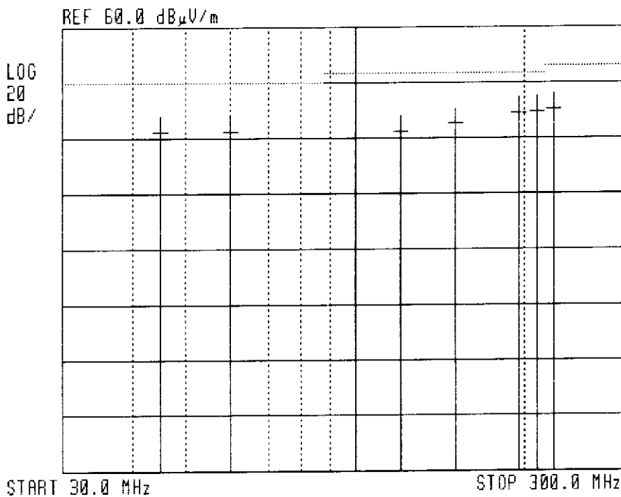
Figure 6.18 Radiated Emission. Antenna Polarisation: Horizontal.
