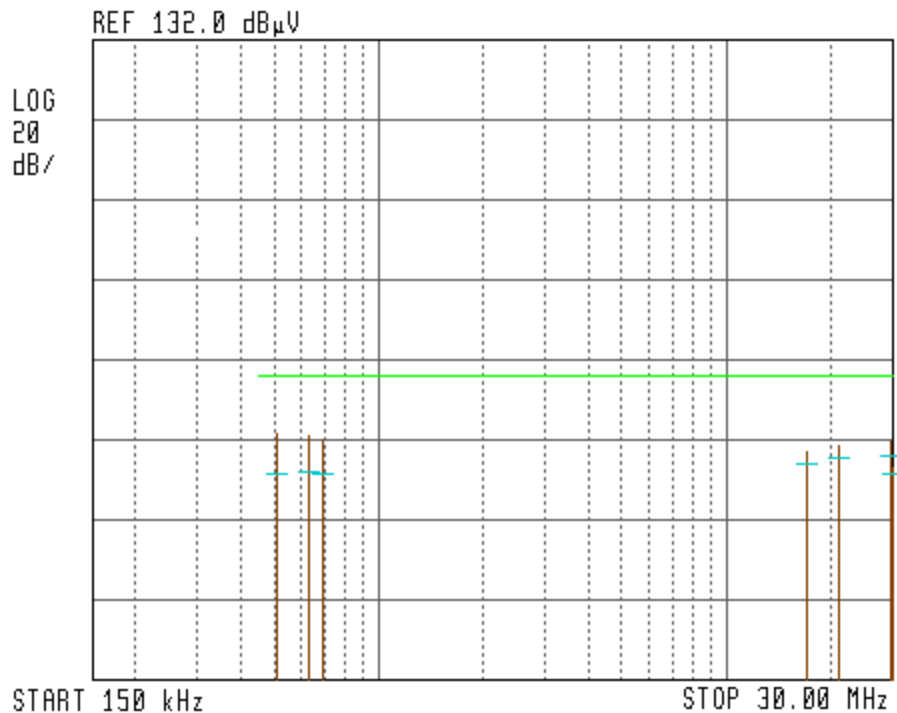
Figure 20 Conducted Emission: NEUTRAL Detectors: Peak, Quasi-peak
