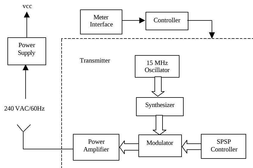
Figure 4. Block Diagram
