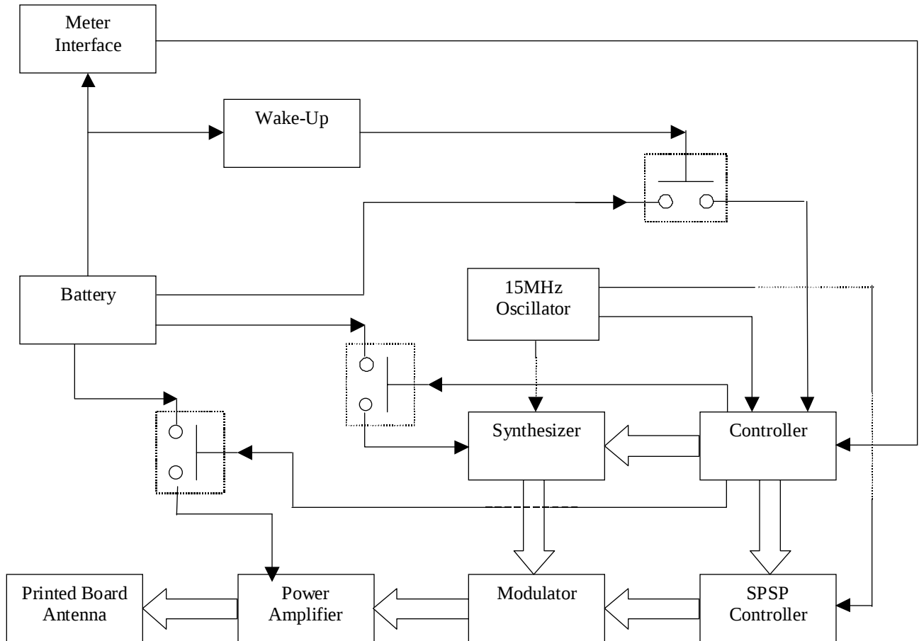
Figure 4. Block Diagram
