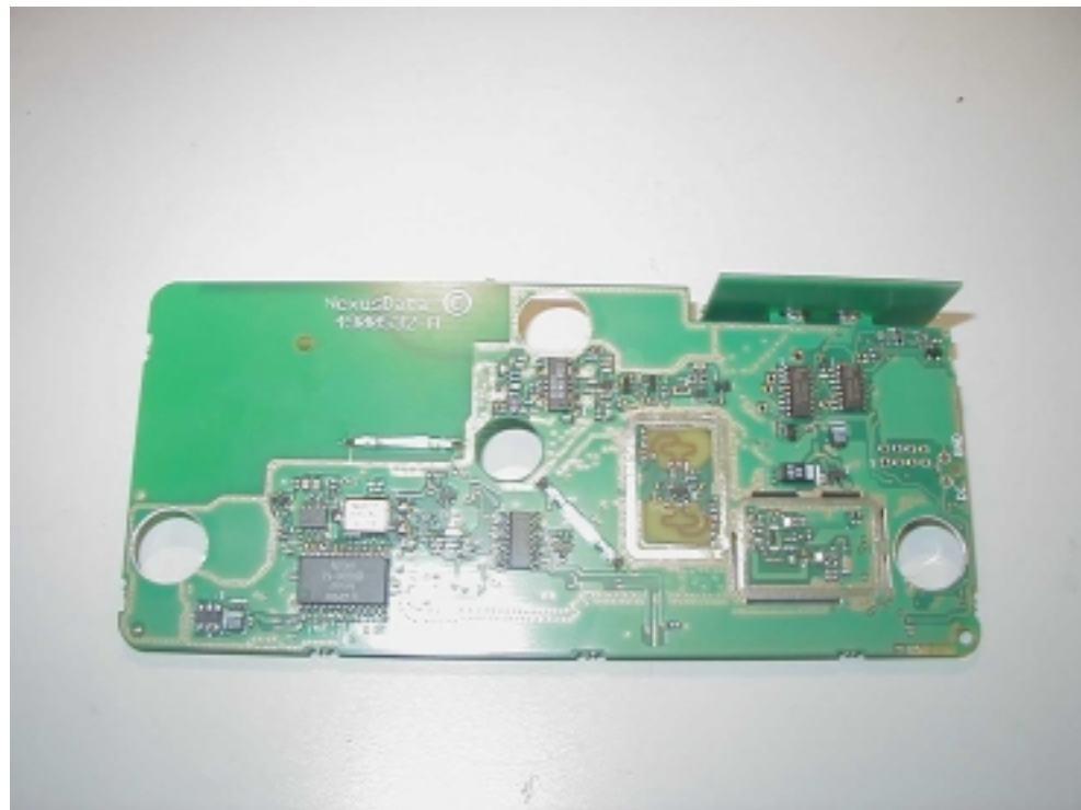
Figure 76 Printed Circuit Side 1
