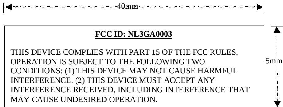
Figure 1. FCC Label
