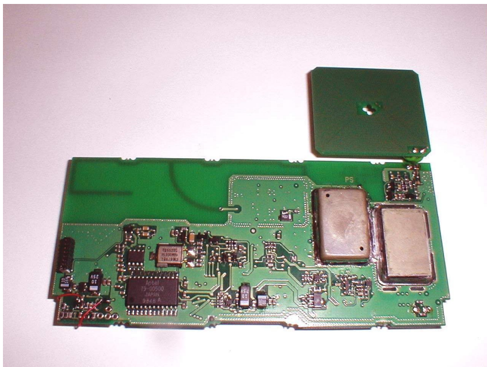
Figure 6 Printed Circuit Side 2
