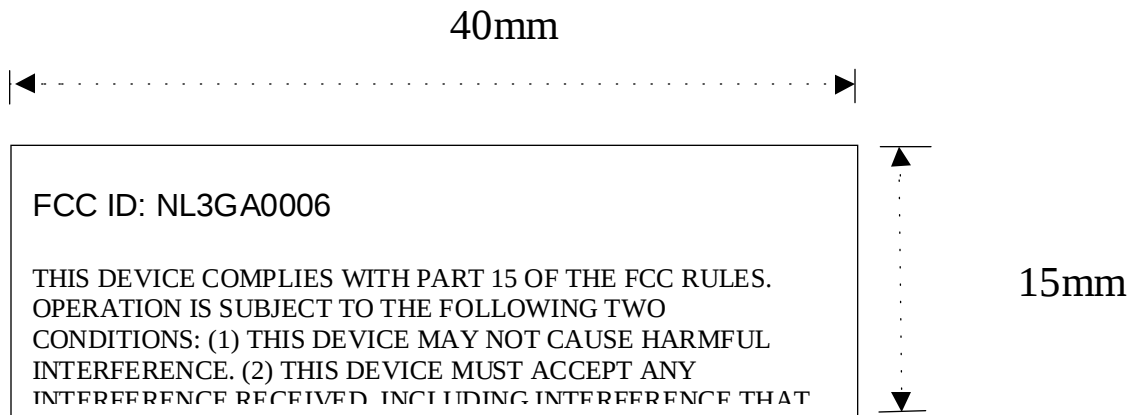
Figure 1. FCC Label
