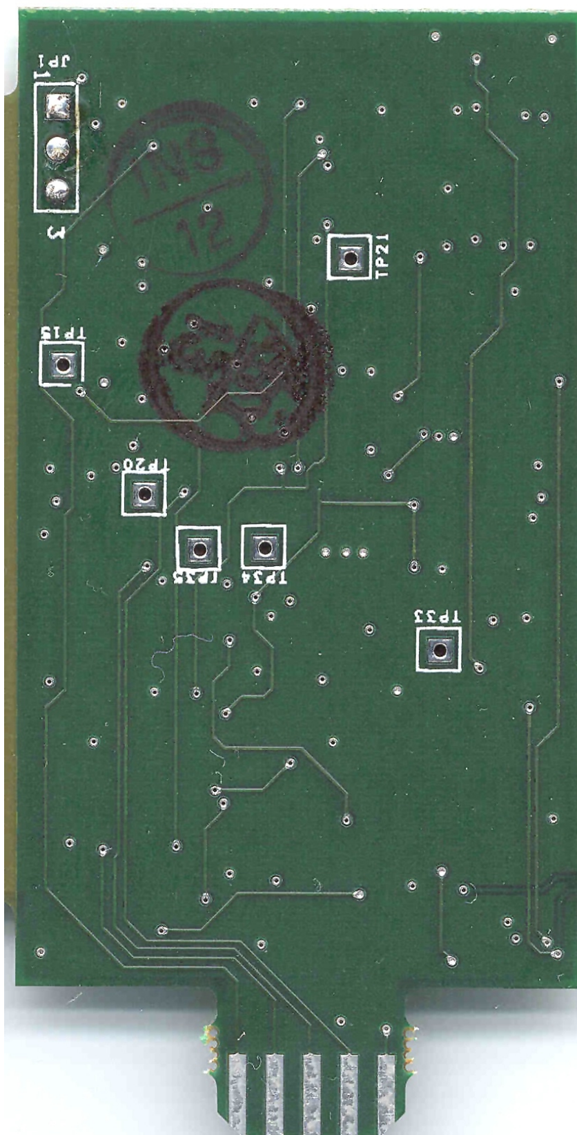
Photo 21. Power Supply and TCXO Portion – Bottom
