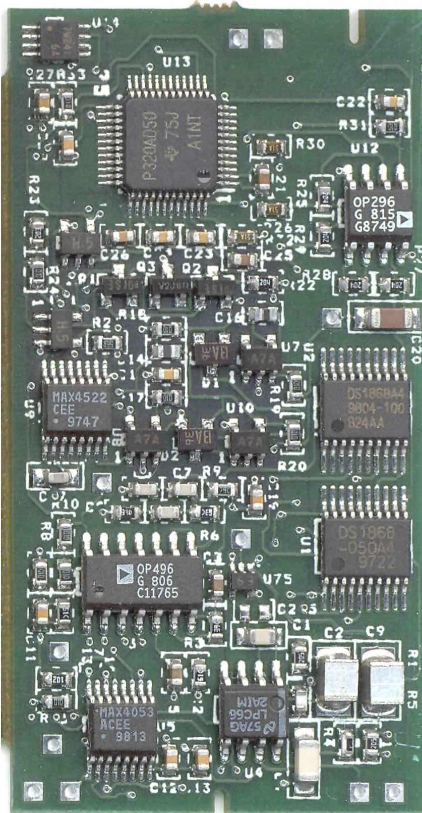
Photo 24. Signal Processing Portion – Top
