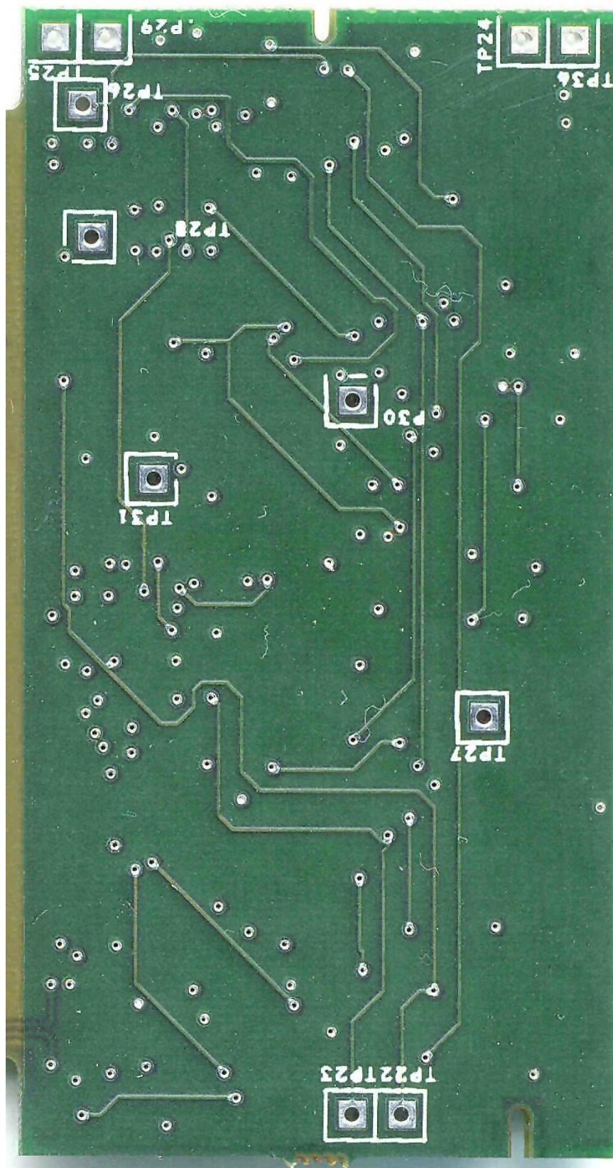
Photo 25. Signal Processing Portion – Bottom
