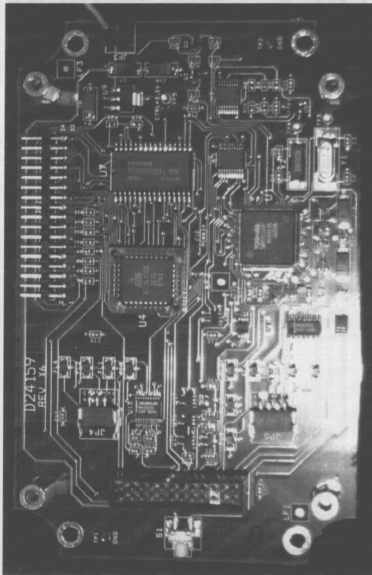
Photo 11. Control Board, Component Side
