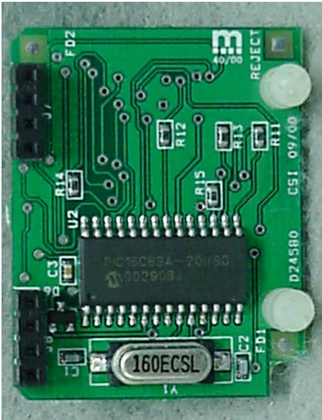
Photo 9. EUT, Bottom View of Transceiver Board
