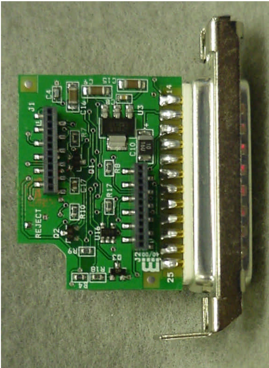
Photo 7. EUT, Bottom View of Power/Protocol Board
