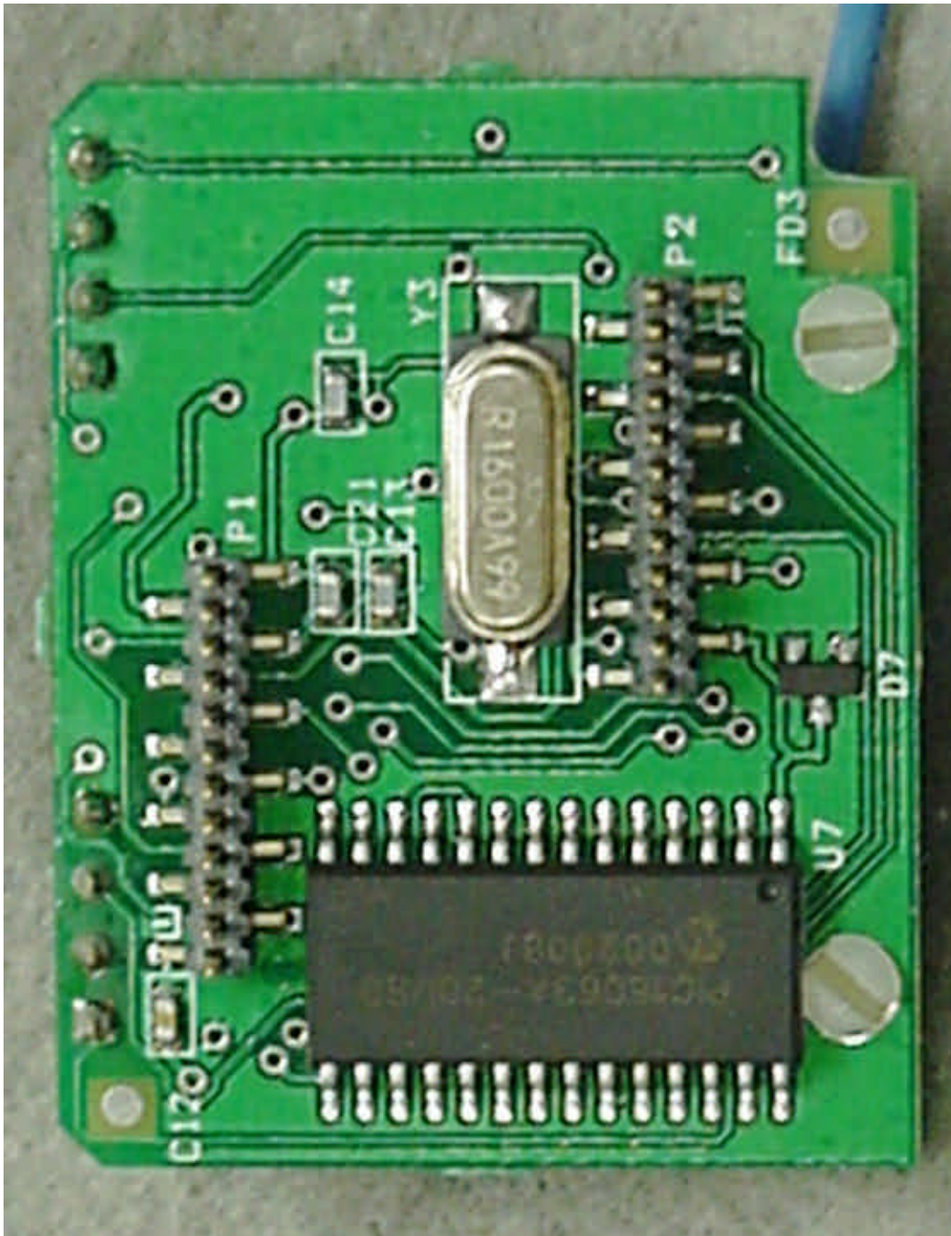
Photo 8. EUT, Top View of Transceiver Board
