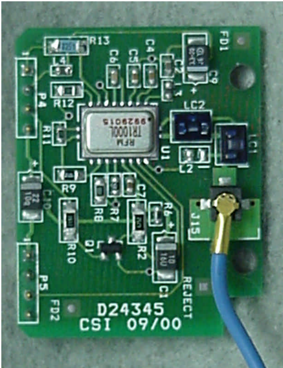
Photo 11. EUT, Bottom View of RF Board
