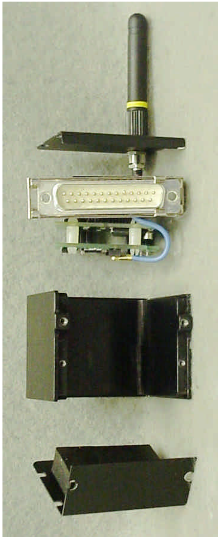
Photo 4. EUT, Exploded View, Front View
