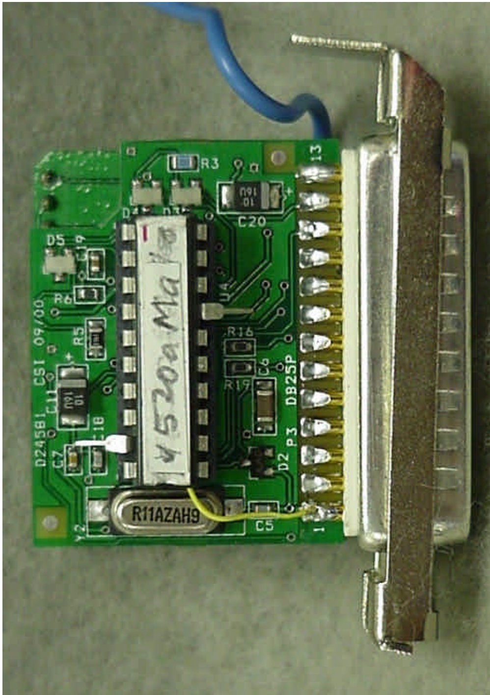
Photo 6. EUT, Top View of Power/Protocol Board
