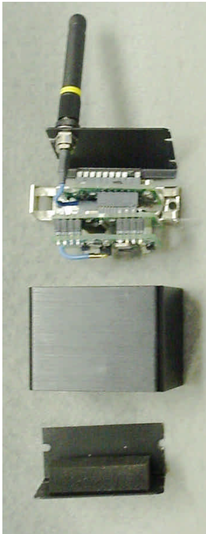
Photo 5. EUT, Exploded View, Rear View
