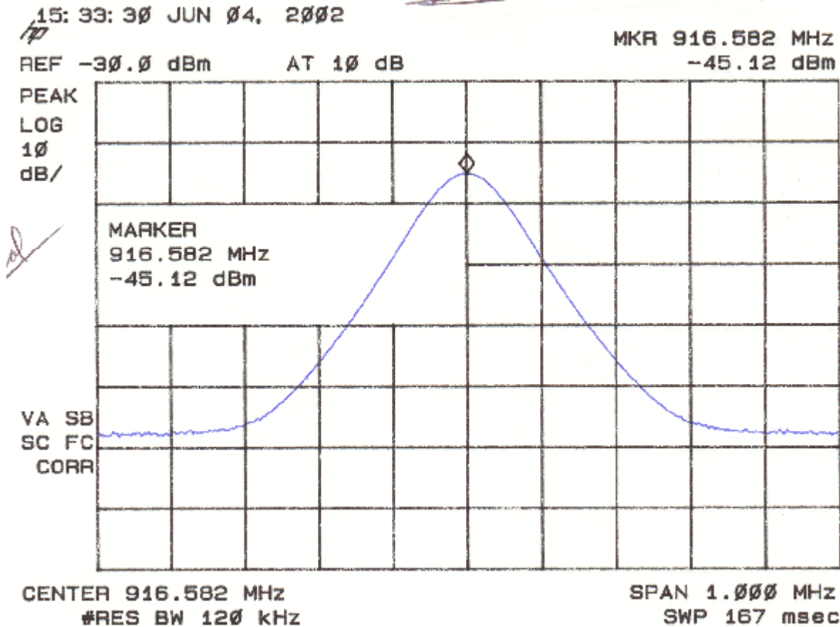
Figure 3 Field Strength of Fundamental Emissions 15.249(a)
