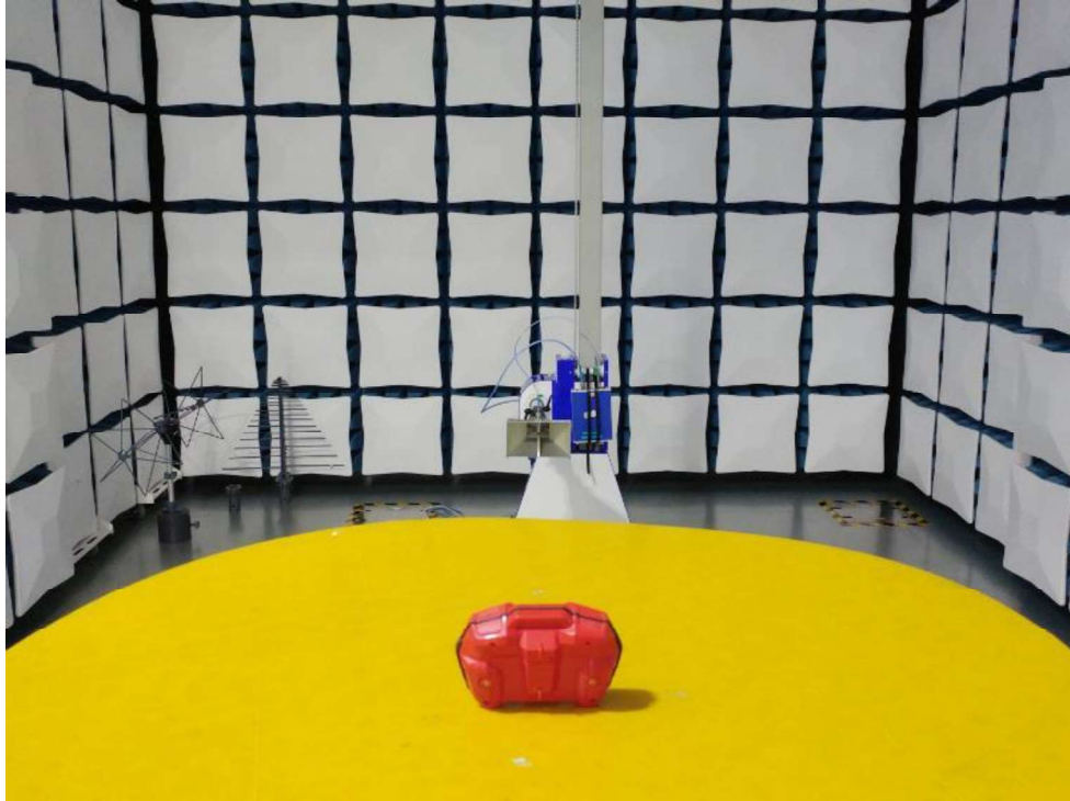
Set-up for Radiated Emission above 1GHz
