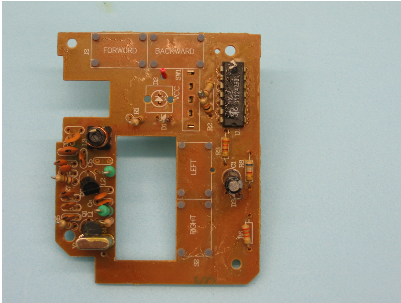
Picture 3 : Transmitter PCB (component side)
