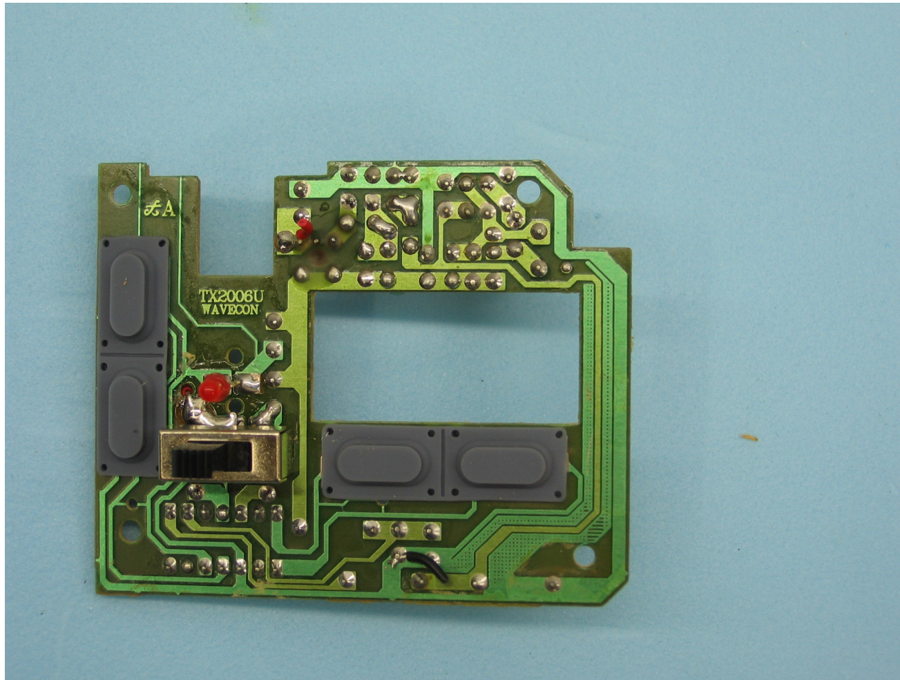
Picture 4 : Transmitter PCB (solder side)
