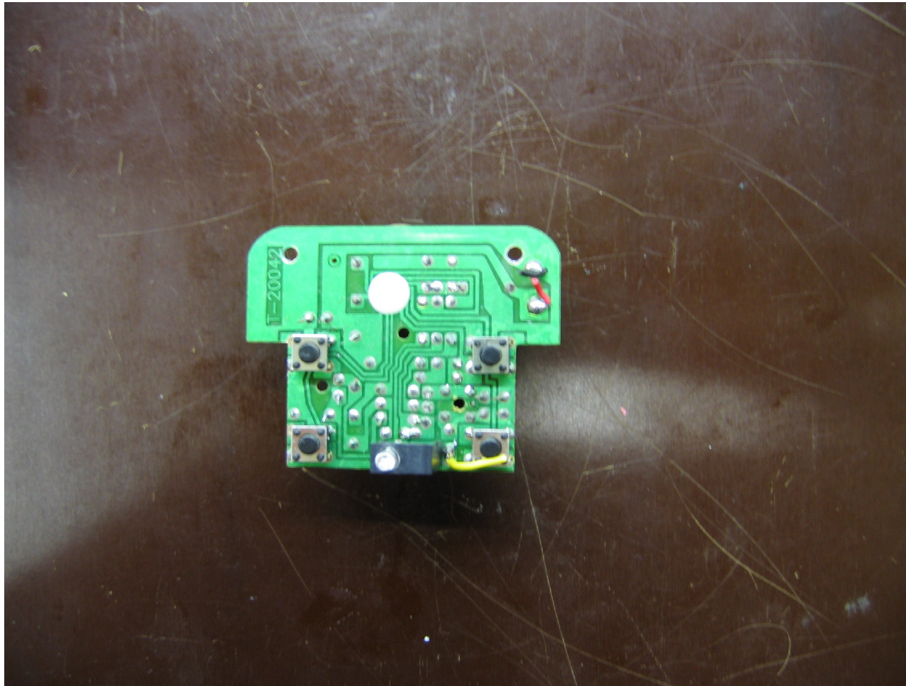
Picture 4 : Transmitter PCB (solder side)
