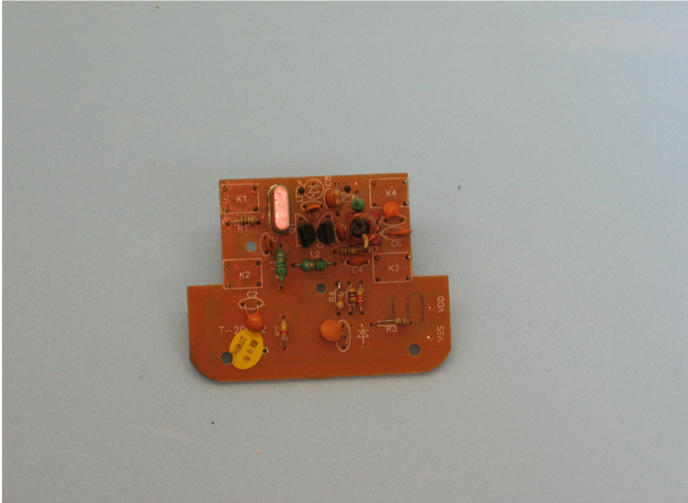
Picture 3 : Transmitter PCB (component side)
