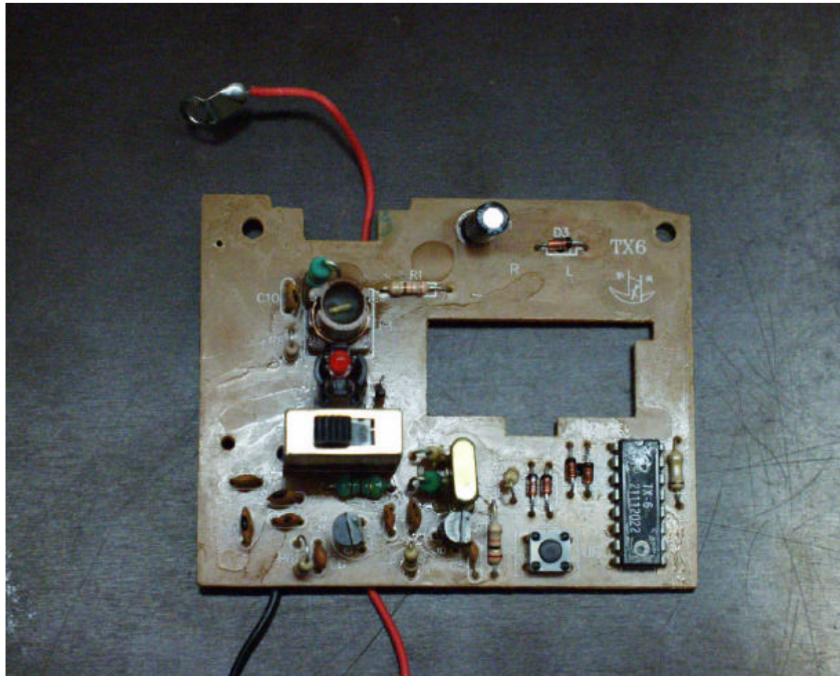
Picture 3 : Transmitter PCB (component side)
