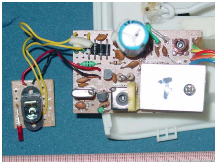
Main PCB
