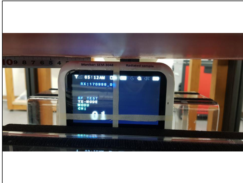
5mm Gap Antenna Folded - Top
