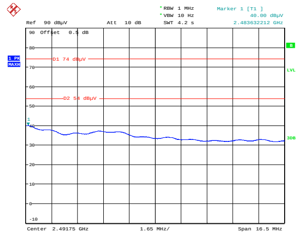
Highest Channel(2 471.625 MHz): AVERAGE
