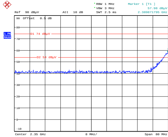
Lowest Channel(2 410.875 MHz): PEAK
