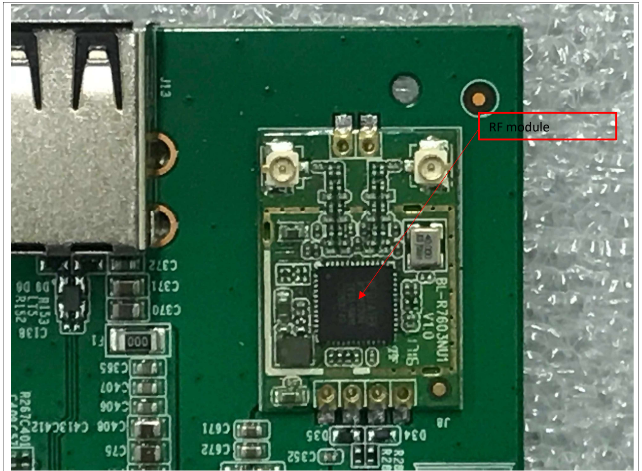
RF chipset
