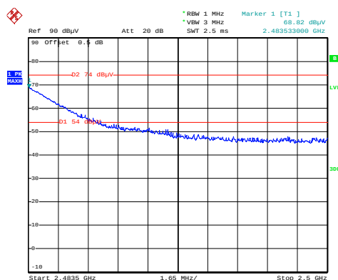
Highest Channel(2 462 MHz): Peak
