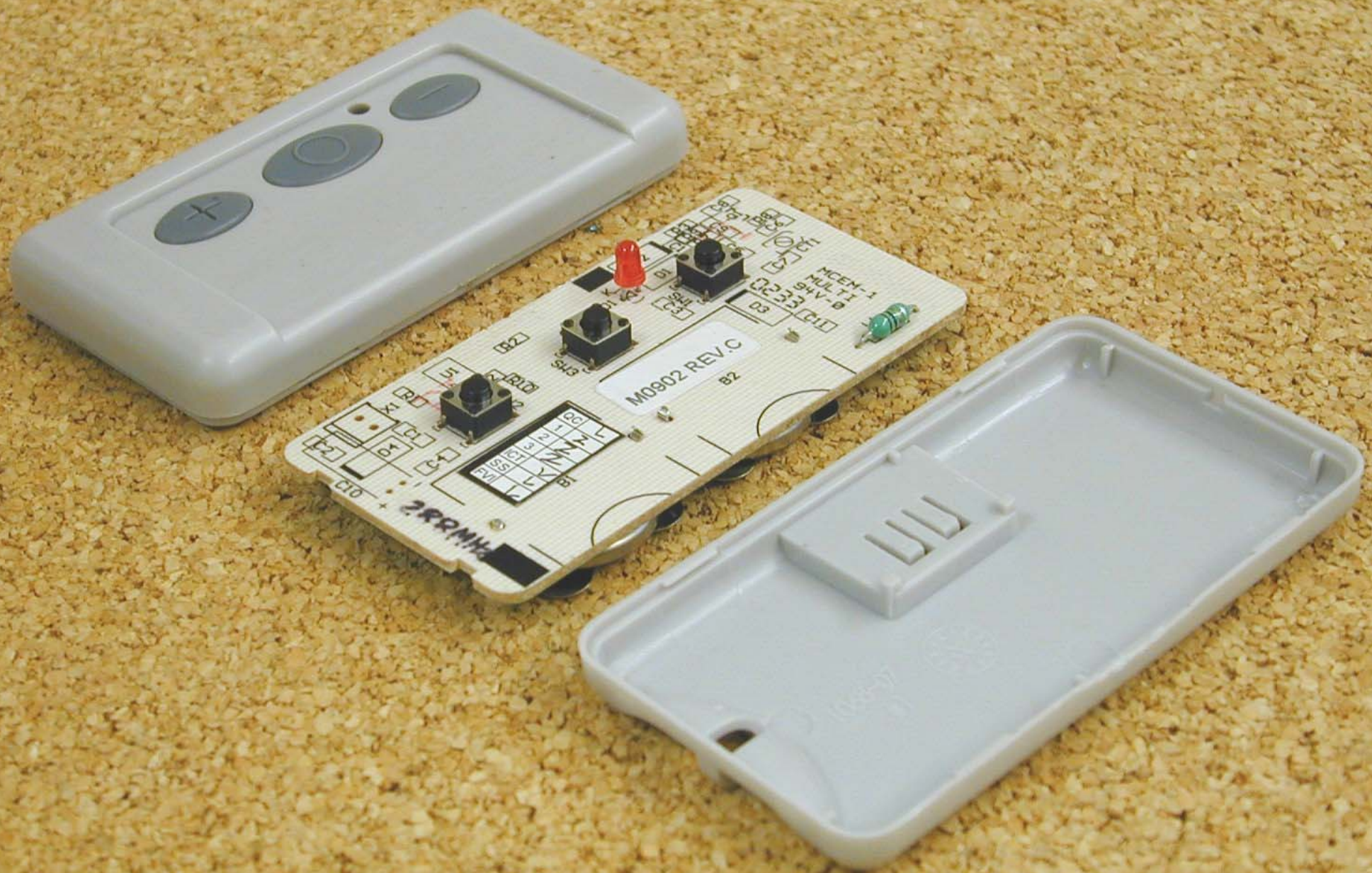
Case Open Bottom View
