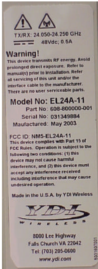
Photograph 1: Unit Label
