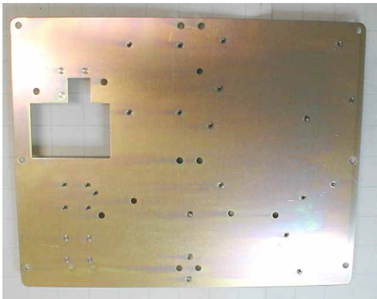
Antenna Bottom
