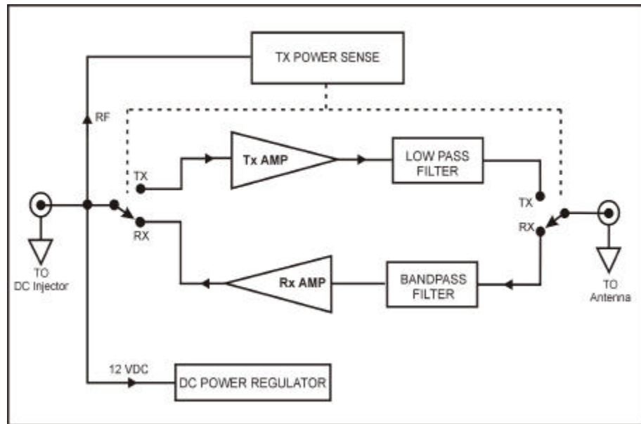
Model 2440 Functional Block Diagram
