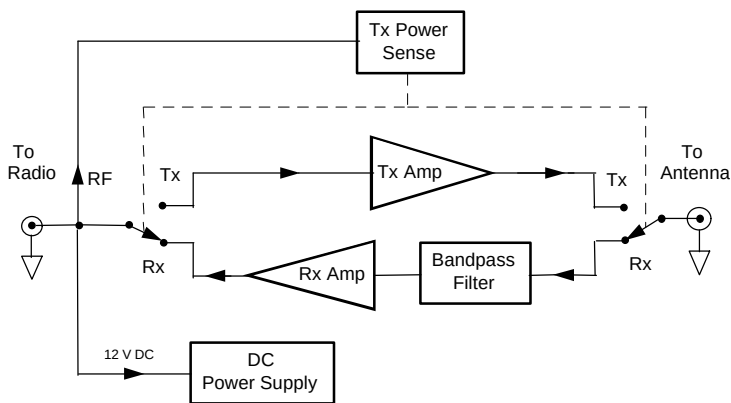
Model 2440 Amplifier Module Functional Block Diagram
