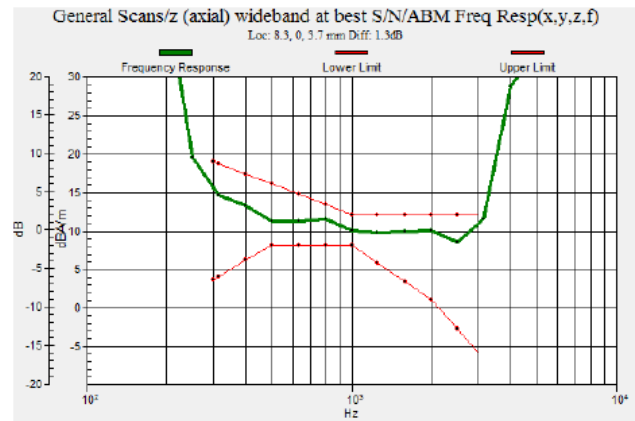
Fig 7.2 GSM1900
