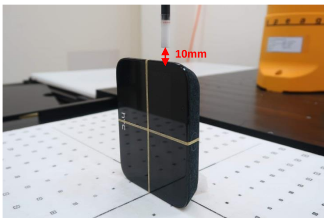
Right Side, Probe sensor to EUT surface distance 10mm
