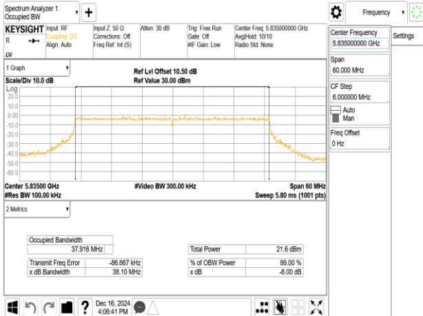
802.11ax_40MHz_Chain0_5835MHz
