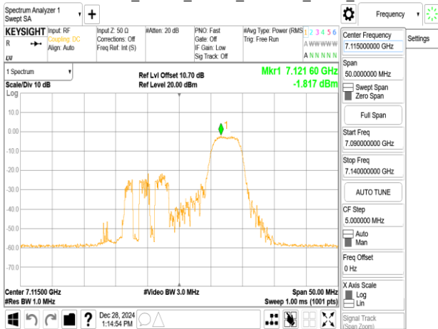
802.11ax_20MHz_Chain0_7115MHz_RU106_54
