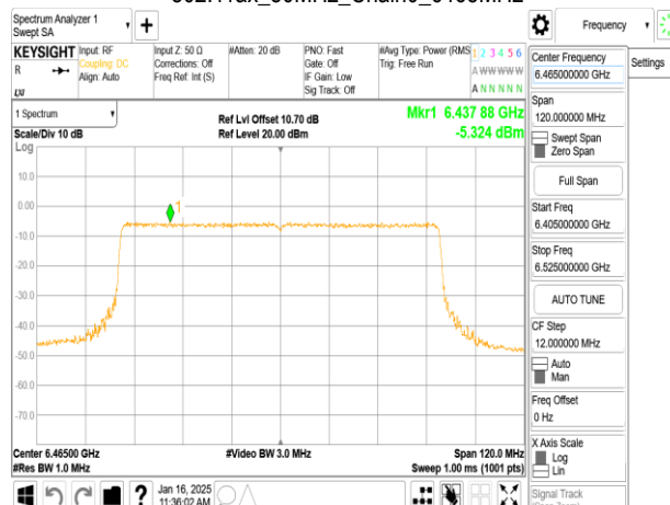
802.11ax_80MHz_Chain0_6465MHz_RU484_65
