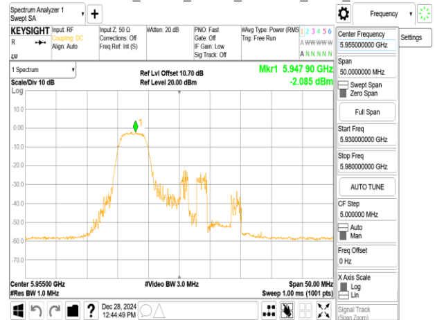
802.11ax_20MHz_Chain0_5955MHz_RU106_53
