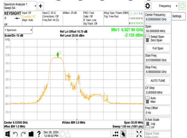
802.11ax_20MHz_Chain0_6535MHz_RU106_53
