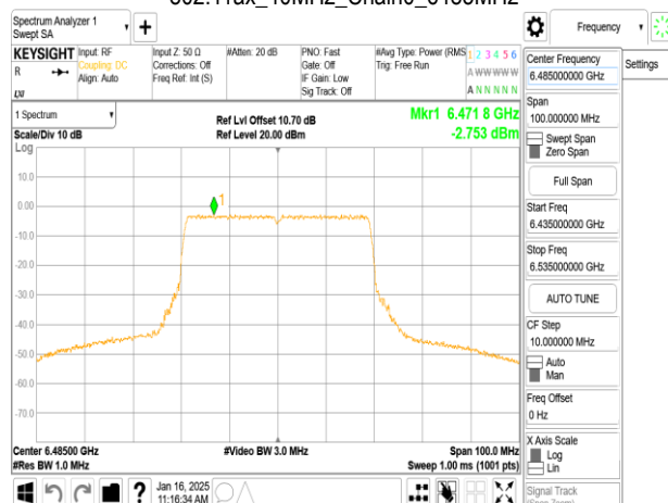
802.11ax_40MHz_Chain0_6485MHz_RU242_62
