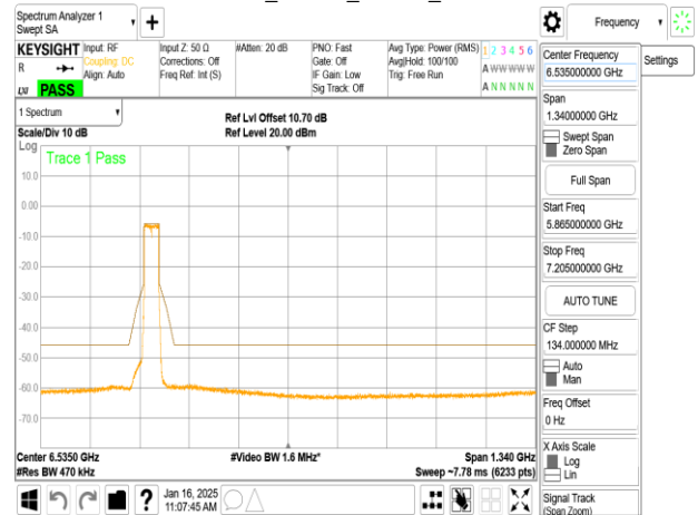
802.11ax_40MHz_Chain0_6405MHz
