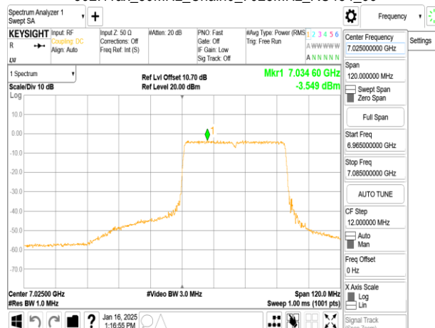
802.11ax_80MHz_Chain0_7025MHz_RU484_66
