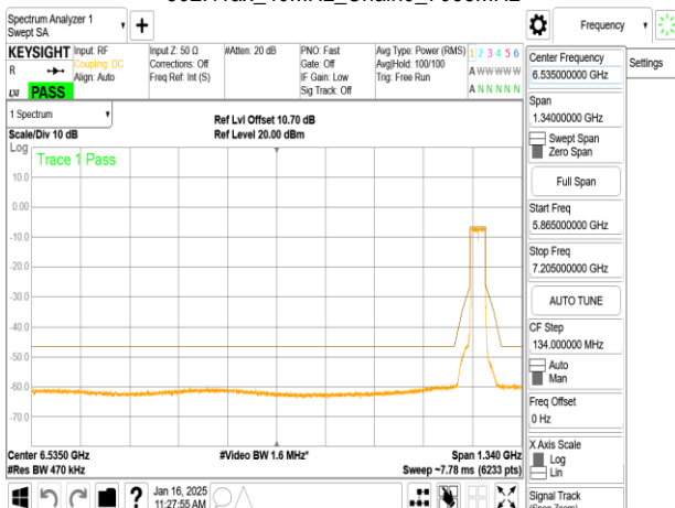
802.11ax_40MHz_Chain0_7085MHz
