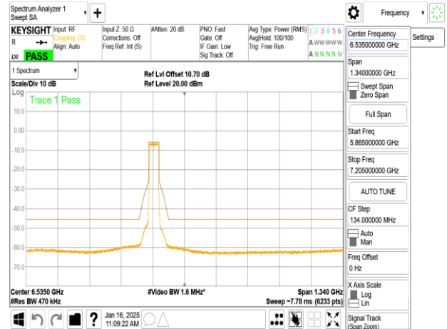
802.11ax_40MHz_Chain0_6445MHz
