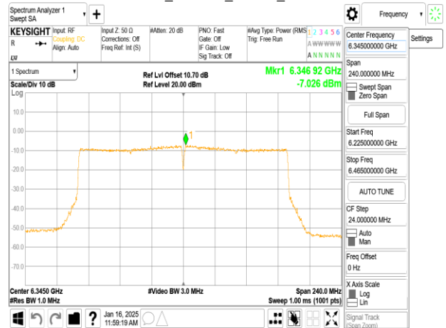
802.11ax_160MHz_Chain0_6345MHz_RU996_S67
