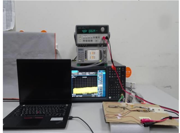
FCC_15_407_WLAN_6E_Conducted_LPI_Setup
