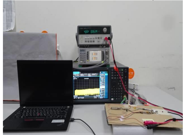
FCC_15_407_WLAN_6E_Conducted_LPI_Setup
