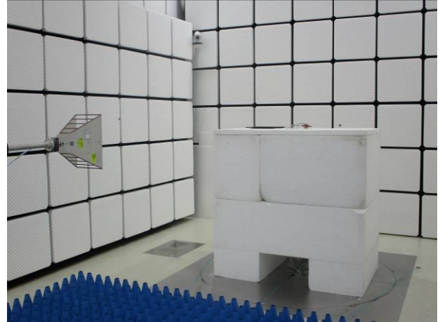
FCC_15_407_WLAN_6E_Radiated_Setup
