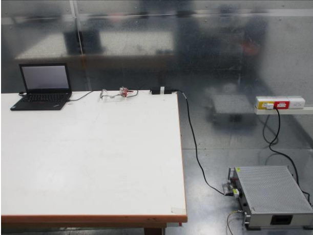
FCC_15_407_WLAN_Conduction_Setup
