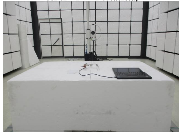
FCC_15_247_WLAN_Radiated_Setup
