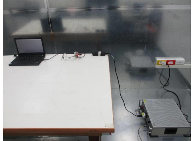
FCC_15_407_WLAN_6E_Conduction_Setup
