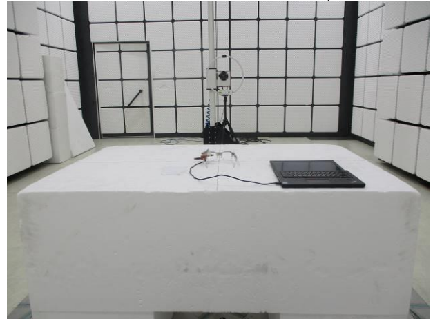
FCC_15_407_WLAN_6E_Radiated_Setup
