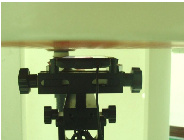
Front Face of the DUT with Phantom 1.0 cm Gap for DUT with Earphone
