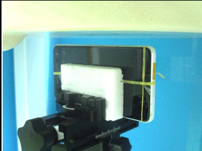
Hotspot - Left Side of EUT at 10 mm
