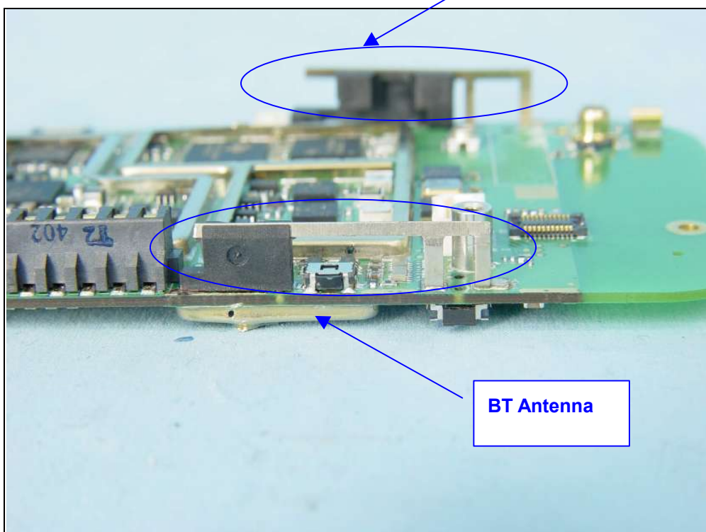
WLAN Antenna
