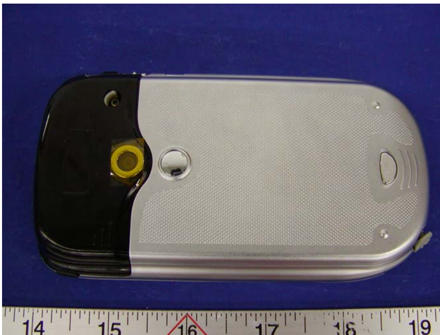
EUT – PH10A Rear View
