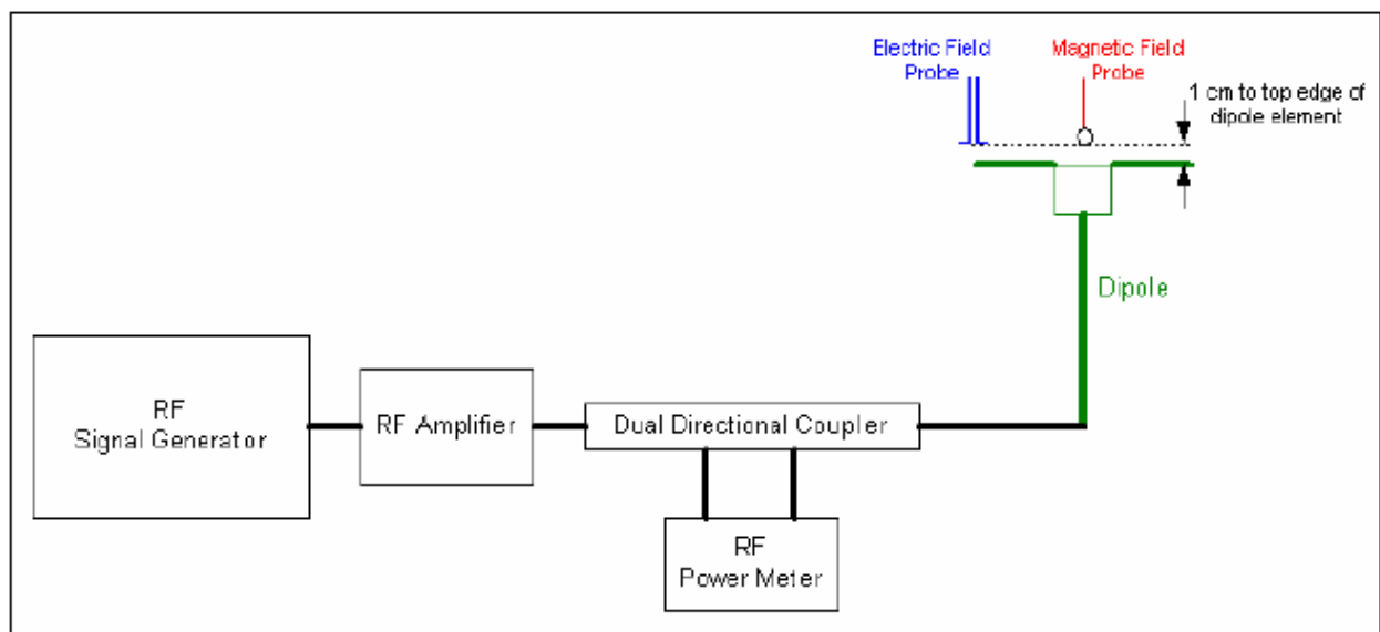
Figure 15: WD dipole calibration procedure
