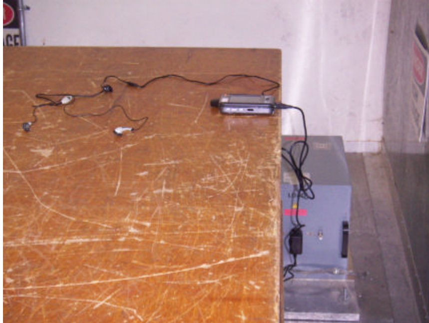
LINE CONDUCTION BACK PHOTO
