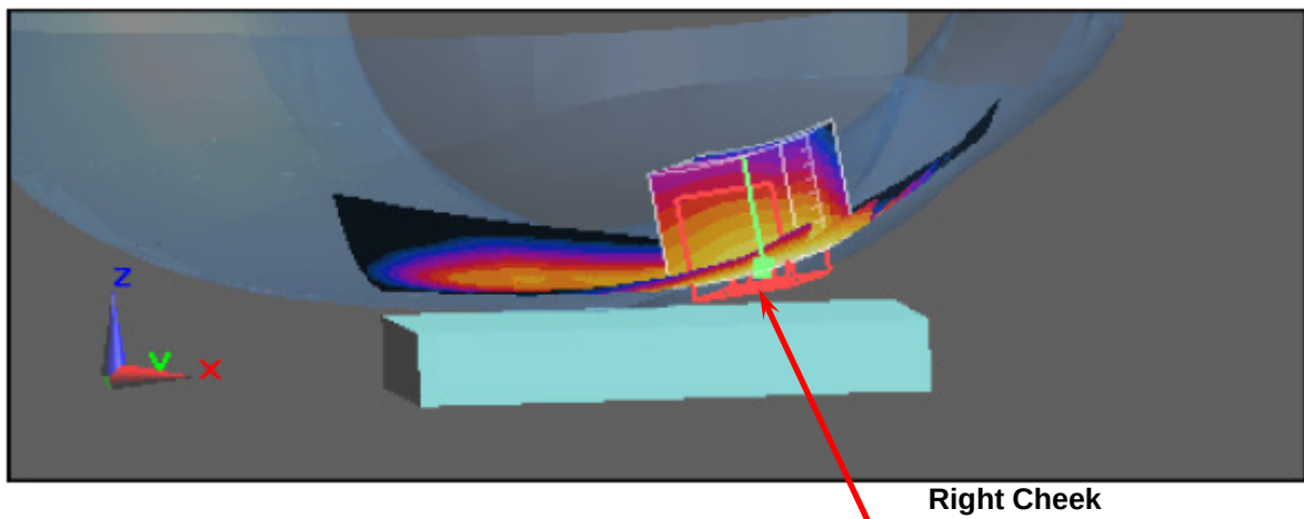
Figure 3. Right Head SAR Test Setup (Cheek) _Open
