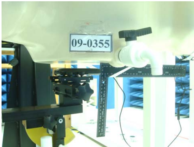
Figure 7. Body SAR Test Setup (Flat Section)_Close
