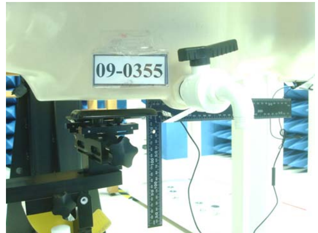
Figure 8. Body SAR Test Setup (Flat Section)_Open
