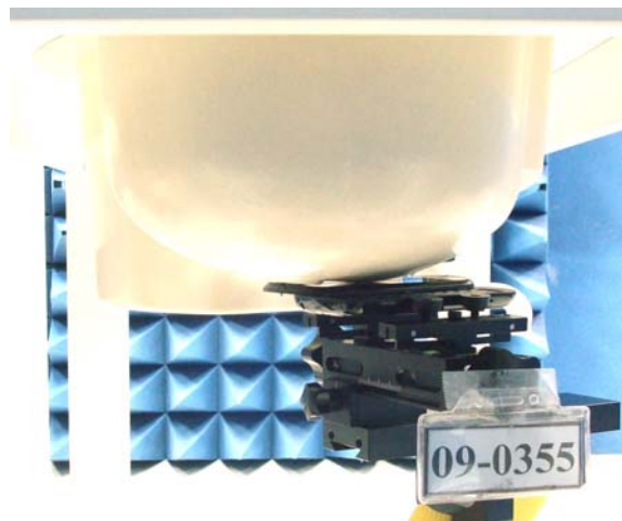
Figure 3. Right Head SAR Test Setup (Cheek) _Open
