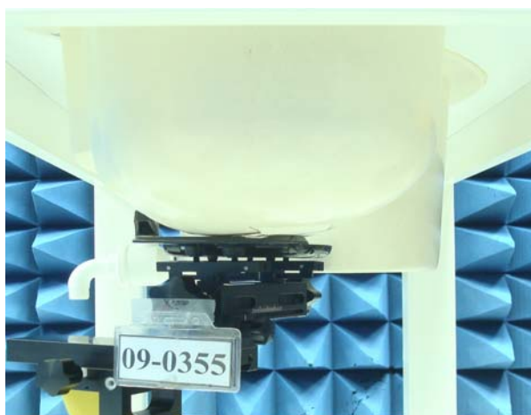
Figure 6. Left Head SAR Test Setup (Cheek)_Open
