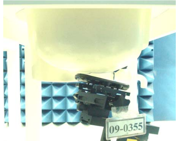
Figure 2. Right Head SAR Test Setup (Tilted) _Close
