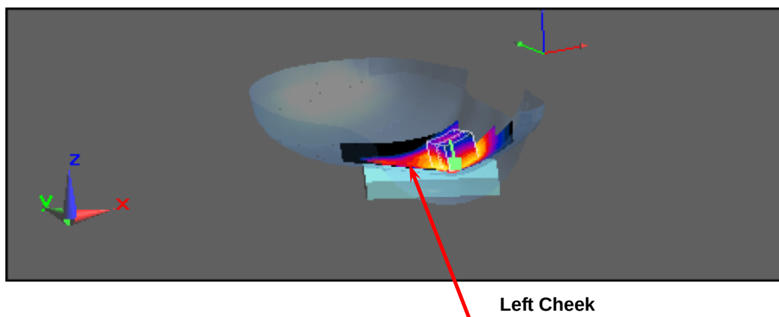
Figure 6. Left Head SAR Test Setup (Cheek)_Open
