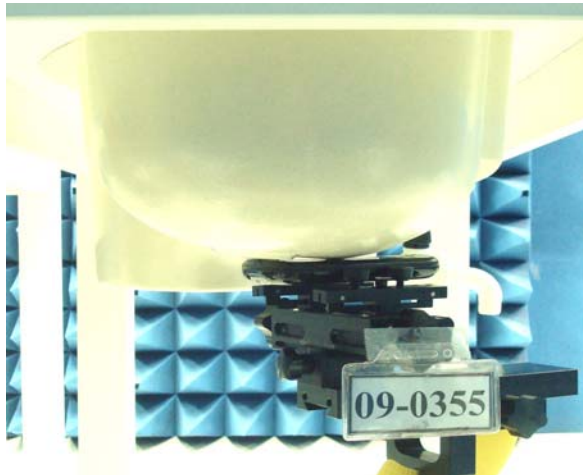
Figure 1. Right Head SAR Test Setup (Cheek) _Close
