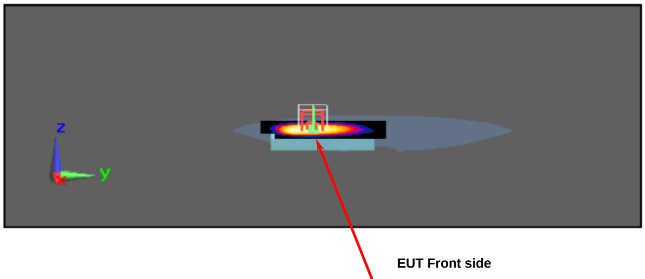
Figure 6. Body SAR Test Setup (Flat Section)
