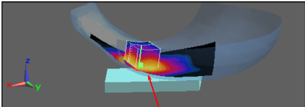
Figure 4. Left Head SAR Test Setup (Cheek)
