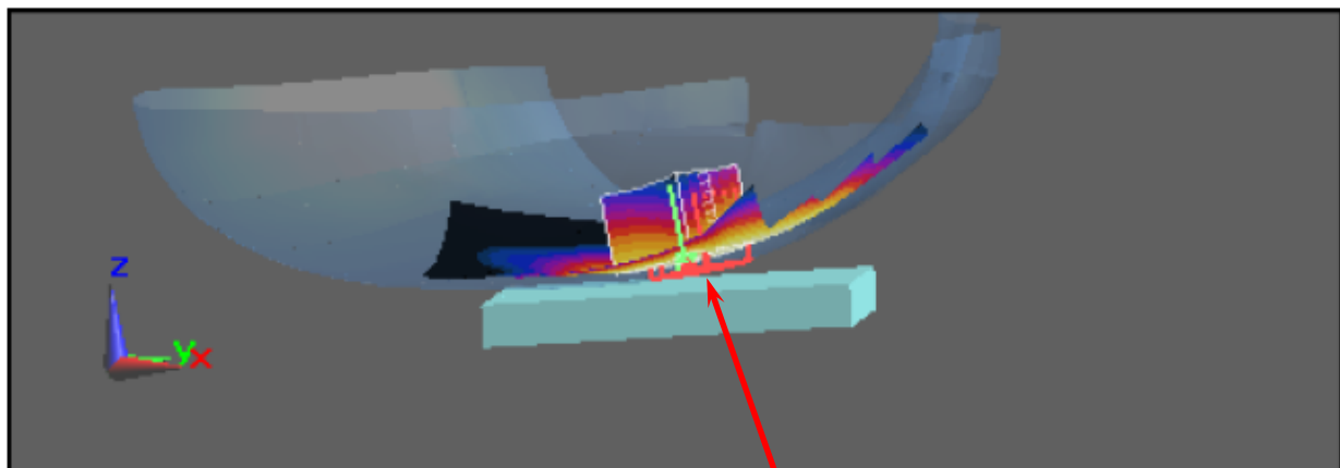
Figure 2. Right Head SAR Test Setup (Cheek)
