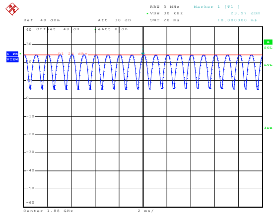
1880MHz - 80% AM
