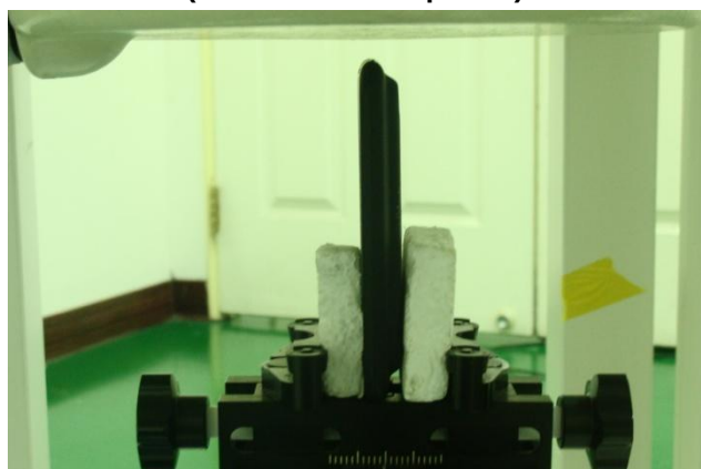
Top Side of the DUT with Phantom 1 cm Gap (DUT without Earphone)
