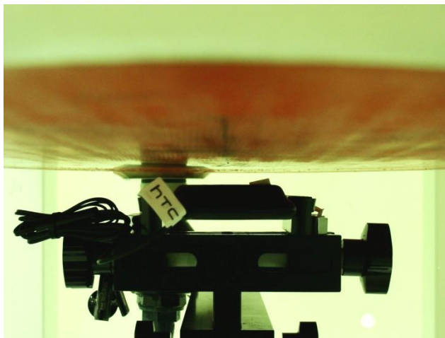
Rear Face of the DUT with Phantom 1 cm Gap (DUT with Earphone)
