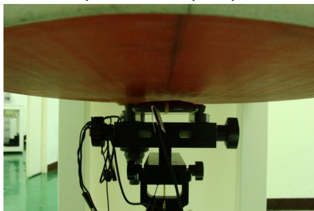
Rear Face of the DUT with Phantom 1.0 cm Gap (DUT with Earphone)
