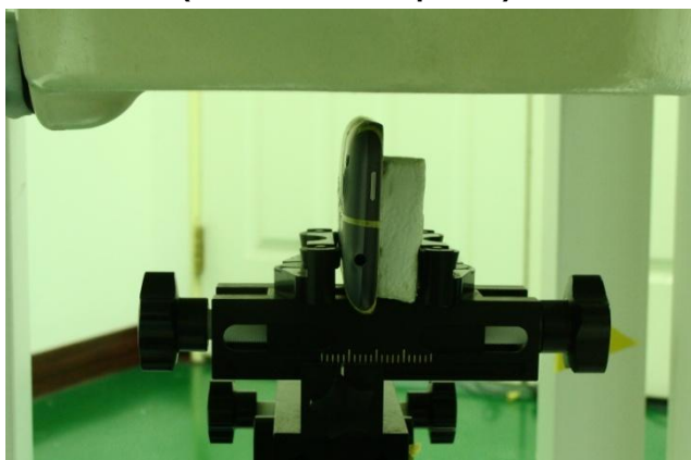
Right Side of the DUT with Phantom 1.0 cm Gap (DUT without Earphone)
