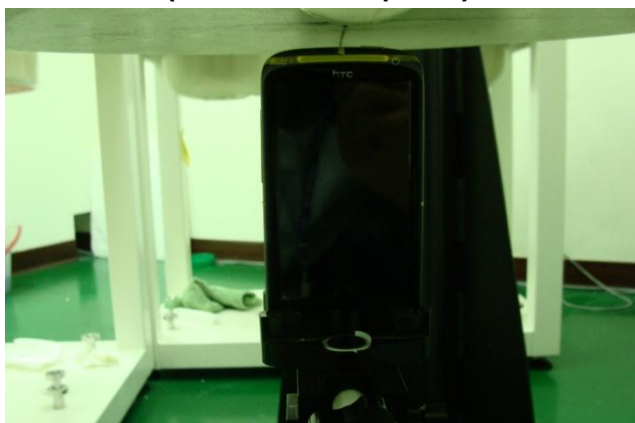
Top Side of the DUT with Phantom 1.0 cm Gap (DUT without Earphone)
