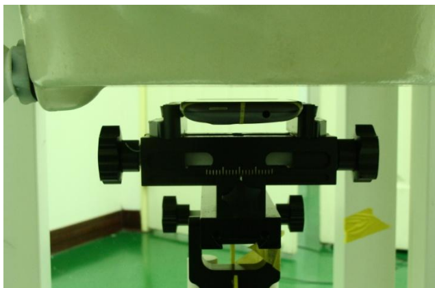
Front Face of the DUT with Phantom 1.0 cm Gap (DUT without Earphone)
