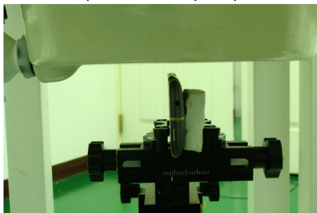
Left Side of the DUT with Phantom 1.0 cm Gap (DUT without Earphone)
