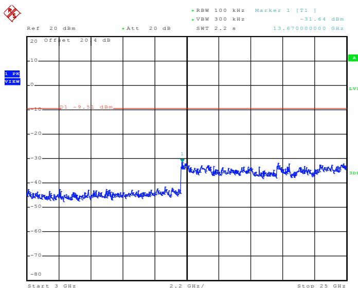
Conducted Spurious Emission Plot between 3 GHz ~ 25 GHz
