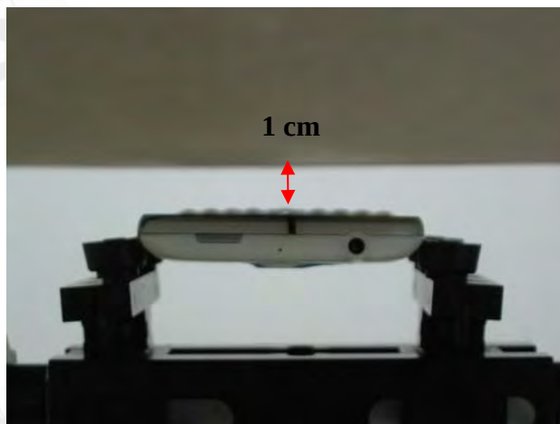
Fig.7 Body worn- EUT front to flat phantom and distance between flat phantom and mobile phone is 1 cm.
