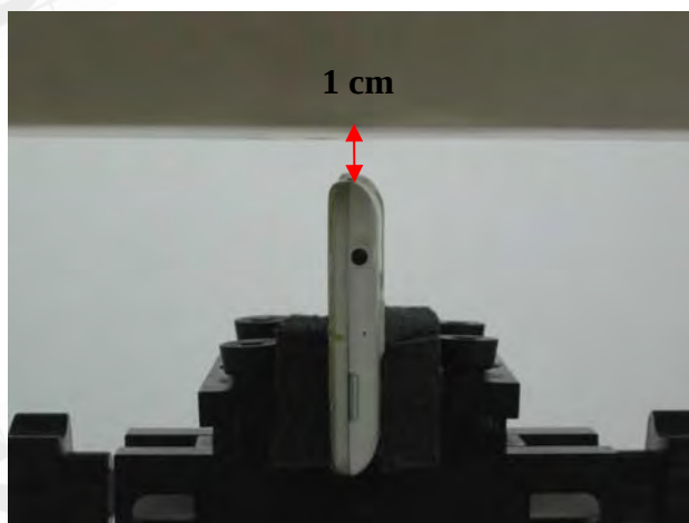
Fig.12 Body worn- EUT Left to flat phantom and distance between flat phantom and mobile phone is 1 cm.
