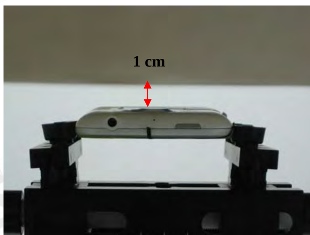
Fig.8 Body worn- EUT back to flat phantom and distance between flat phantom and mobile phone is 1 cm.
