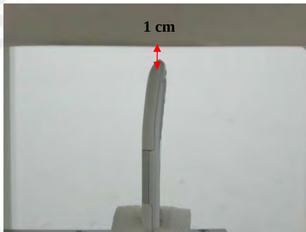
Fig.9 Body worn- EUT Top to flat phantom and distance between flat phantom and mobile phone is 1 cm.
