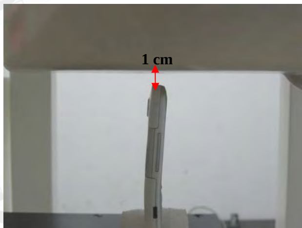
Fig.10 Body worn- EUT Bottom to flat phantom and distance between flat phantom and mobile phone is 1 cm.
