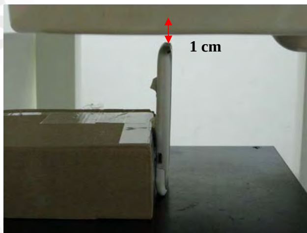
Fig.9 Hotspot mode- EUT Top to flat phantom and distance between flat phantom and mobile phone is 1 cm.
