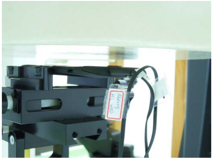
Rear Face of DUT with 1 cm Gap (Body Worn, EUT + Earphone 1)
