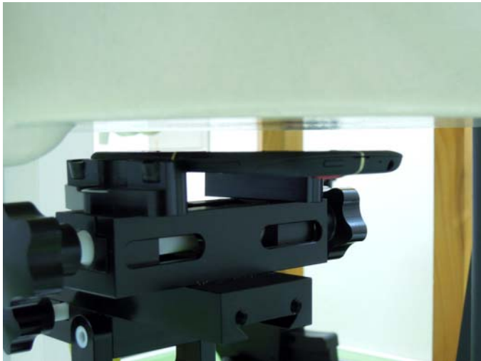
Front Face of DUT with 1 cm Gap (Hotspot Mode)
