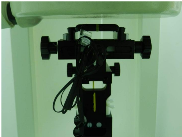
Back of the DUT with Phantom 1 cm Gap (DUT with Earphone 2)
