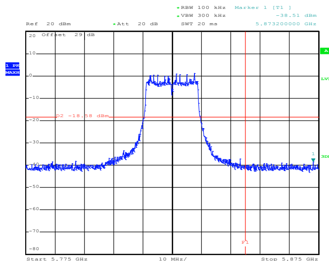
High Band Edge Plot on 5GHz 802.11n HT20 Channel 165
