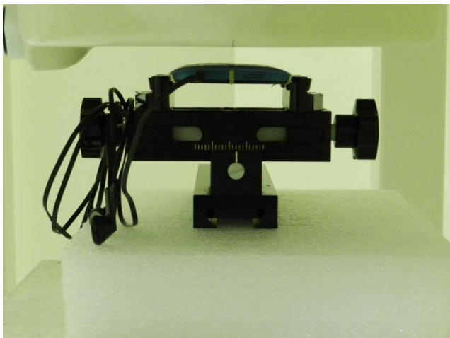
Back of the DUT with Phantom 1 cm Gap (DUT with Headset)
