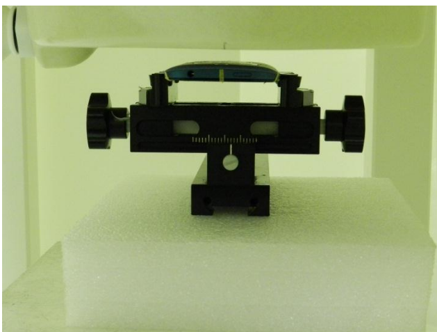
Back of the DUT with Phantom 1 cm Gap (DUT without Headset)
