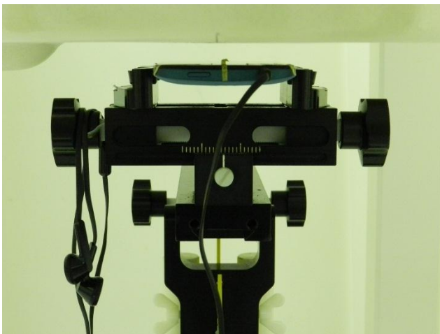
Front of the DUT with Phantom 1 cm Gap (DUT with Headset)
